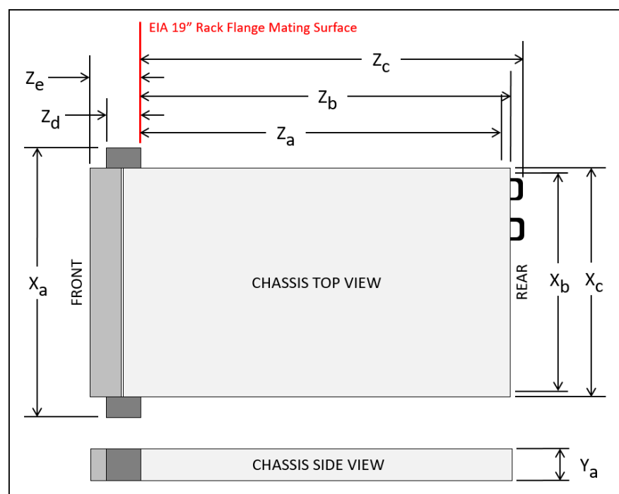
Figure 8. Server dimensions
