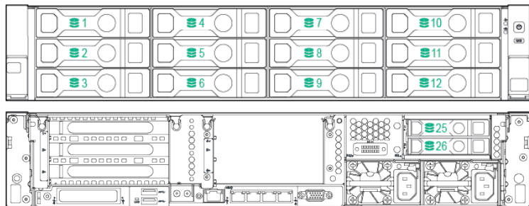
12 LFF + 2 rear SFF hot-plug drive model
