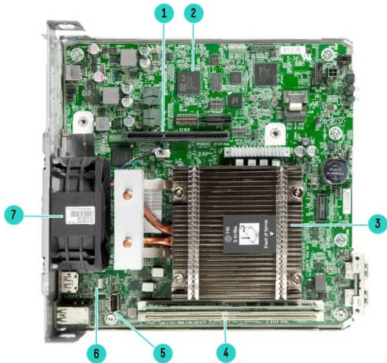
HPE ProLiant MicroServer Gen10 Plus Mainboard Internal View:
